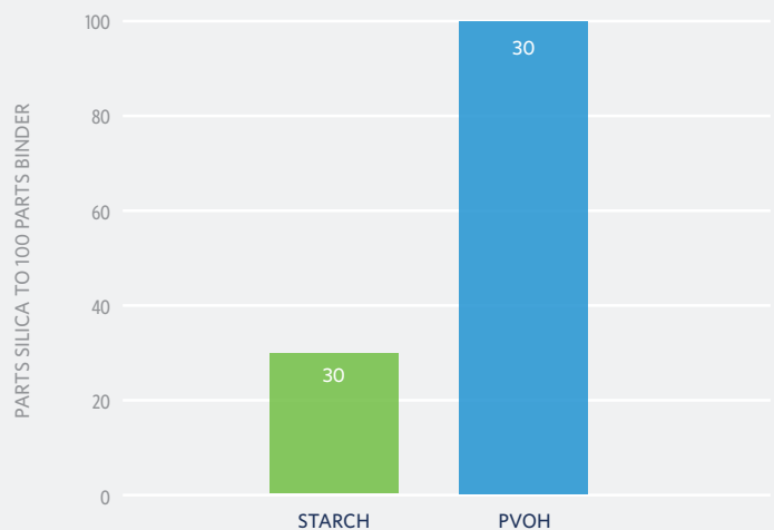
FIGURE 1: Maximum Silica Loading Prior to Dusting Silica Surface Area - 260 m 2 /gm
