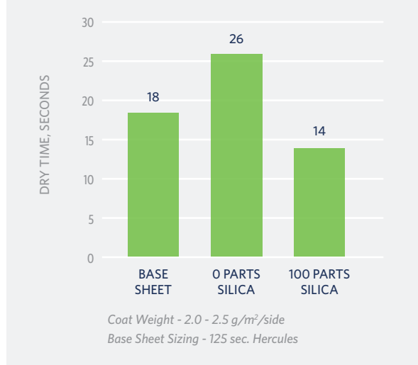
FIGURE 3: Hewlett Packard Dry Time with Selvol 107
